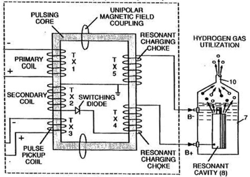
VOLTAGE INTENSIFIER (VIC) CIRCUIT (FIG. 10)
