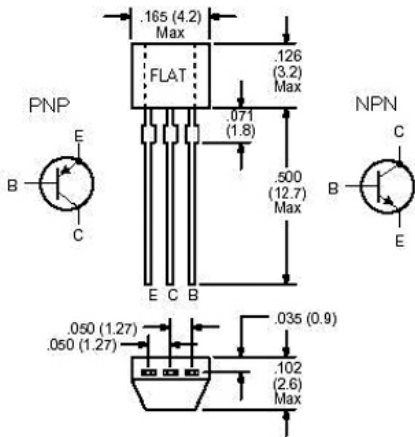
NTE2361 (NPN) & NTE2362 (PNP) Silicon Complementary Transistors High Speed Switch
